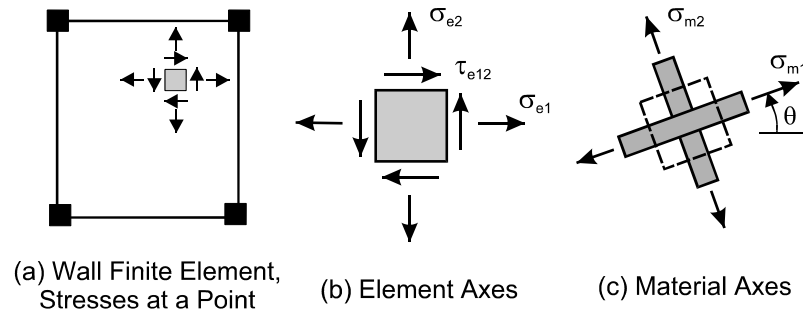
Figure 4 Initial and Principle Material Axes
