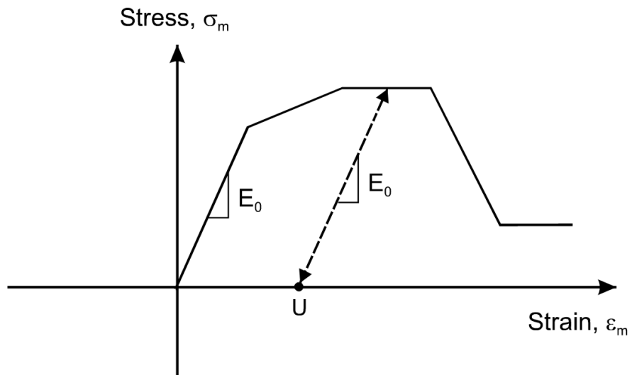
Figure 2 Unloading-Reloading Behavior
