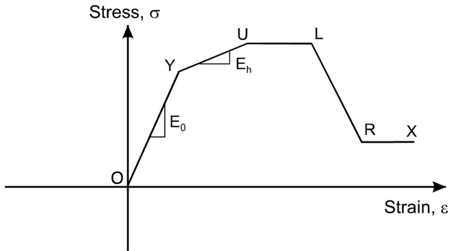
Figure 1 Uniaxial Stress-Strain Relationship
