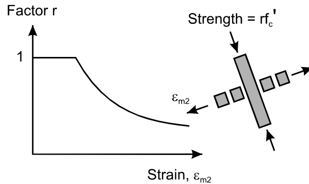
Figure 5 Reduction in Compression Strength Due to Tensile Strain in the Perpendicular Direction
