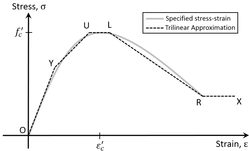
Figure 3 Trilinear Approximation of Concrete Stress-Strain Curve
