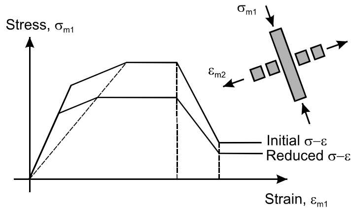
Figure 6 Change in Stress-Strain Relationship to Account for Strength Reduction
